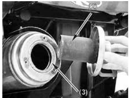
(2) Spark Arrester
