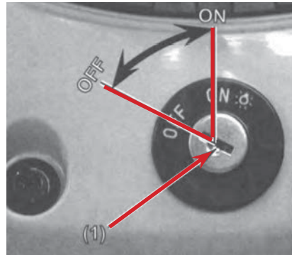
(1) Ignition switch
