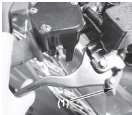
1. Parking Brake (Brake Lever Lock)
